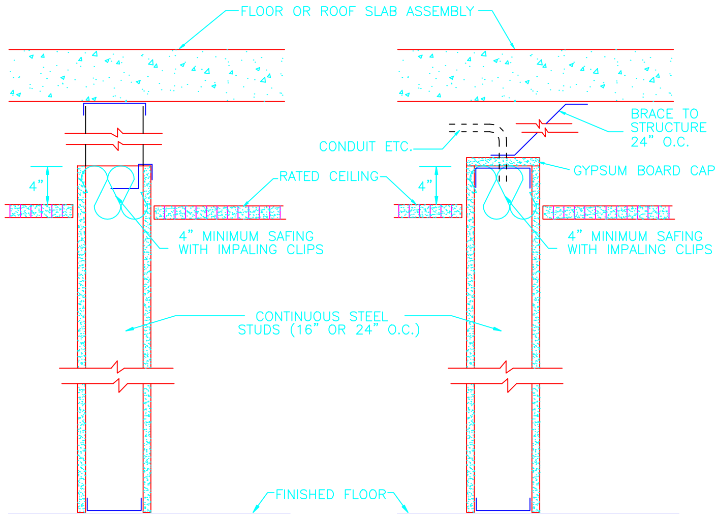
NON-RATED PARTITION THRU A RATED CEILING ASSEMBLY - DYNAMIC
